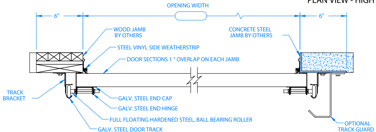
PLAN VIEW - HIGH LIFT
