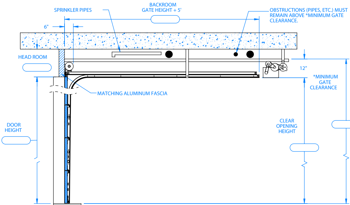
SECTION ELEVATION
