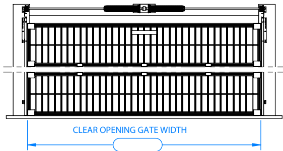
INTERIOR ELEVATION
